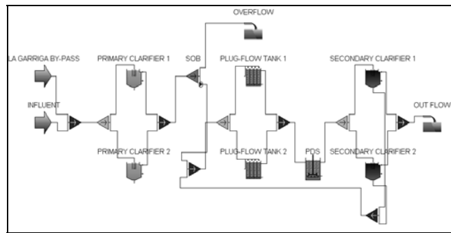
Fig. 6. Layout of the Granollers WWTP in GPS-X
