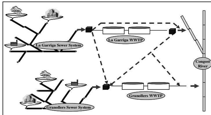
Fig.2. Main elements of the system
