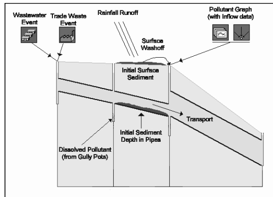
Fig. 5. Components of the water quality module
